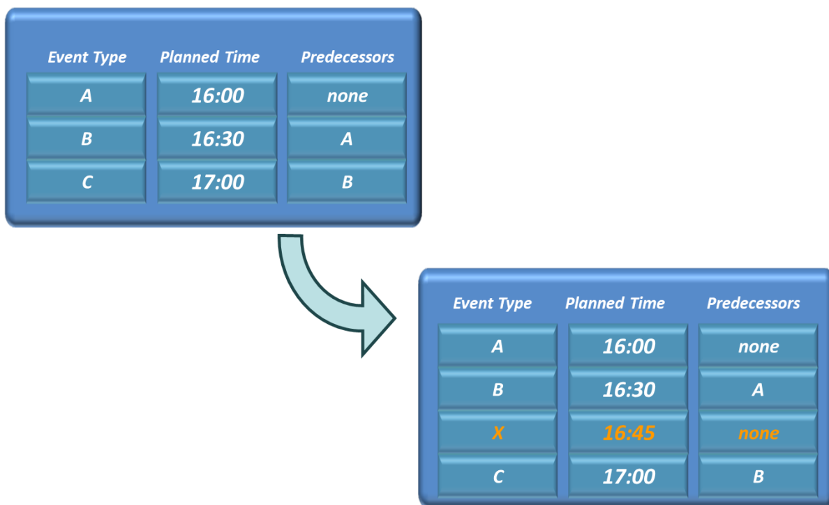
DIAGRAM 9 - EVENT INSERTION
