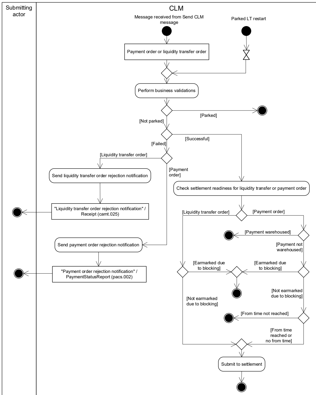
Figure 47 - Process CLM payment order and liquidity transfer order
