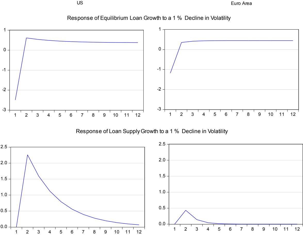
Figure 8: Simulation Analysis
