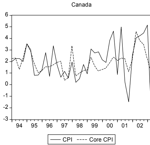
Figure 2: Inflation Rates
